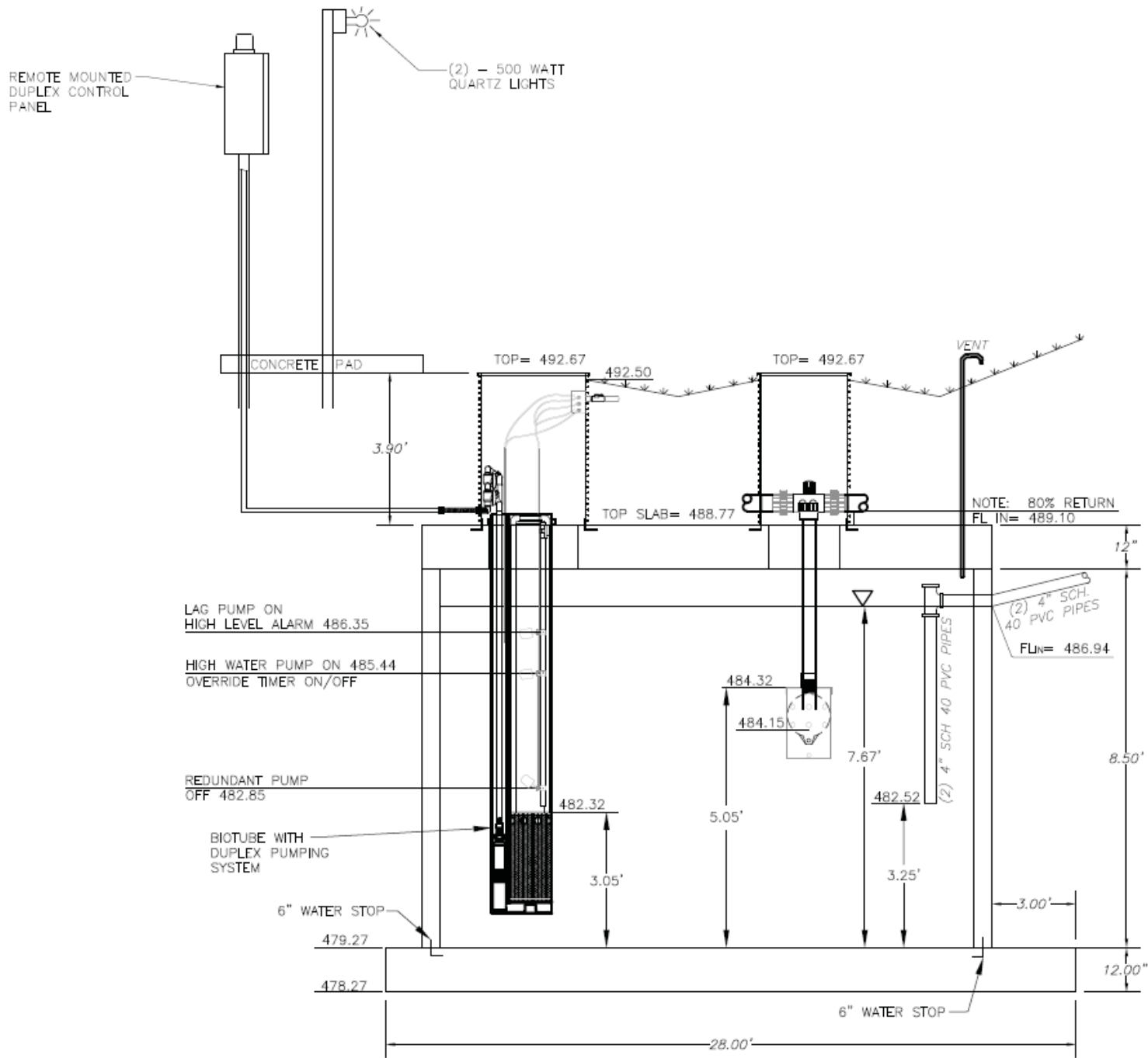
75,000 GALLON RECIRCULATION TANK N.T.S.
